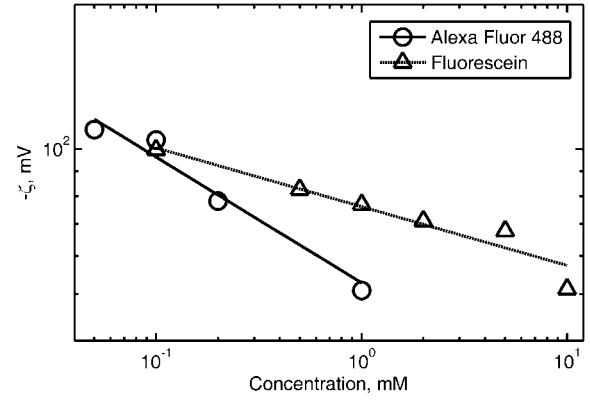
Figure 3. Zeta potential measurement results versus Alexa Fluor 488 and sodium fluorescein concentration. A power law fit of the form \zeta = -aC^b gave a = 0.0527 \text{ V/mM}^b and b = -0.261 for Alexa Fluor 488 and a = 0.0760 \text{ V/mM}^b and b = -0.122 for Fluorescein. Data are shown over the concentration range used in CP experiments.
